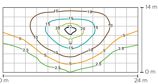
LUMINARIA INDIVIDUAL
